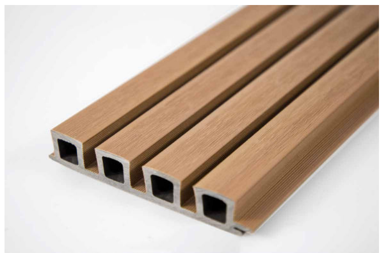
Engineered polymer cap with bamboo PE composite core
